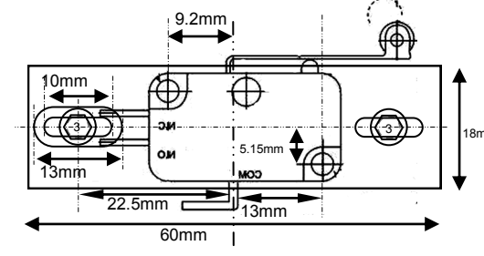
V5 microswitch carriers (Y) 5mm aluminium
