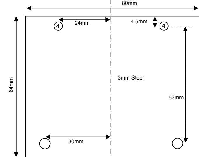
Read head carrier 3mm steel
