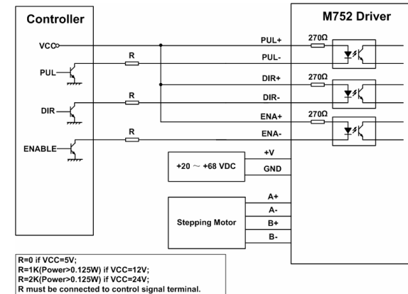
Figure 10: Typical connection
