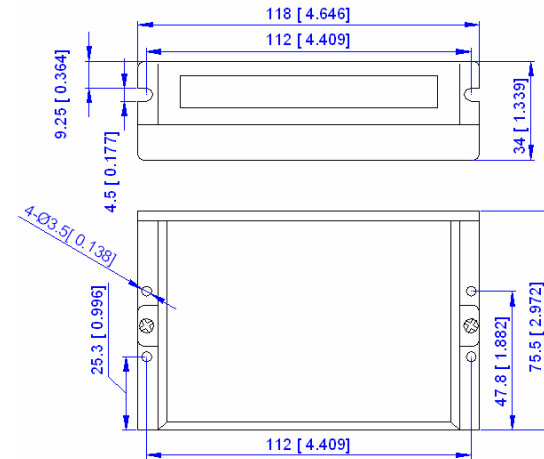
Figure 1: Mechanical specifications
