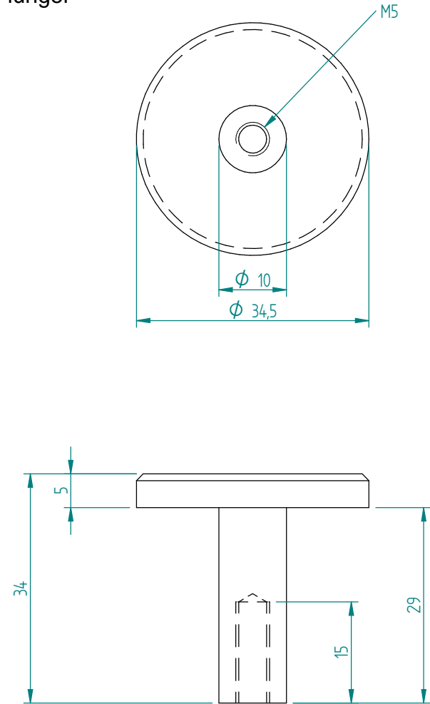
Plunger
